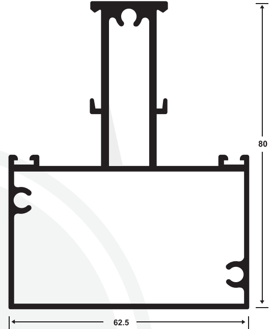
3602 MARCO CENTRAL
