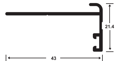
3610 TOPE CENTRAL
